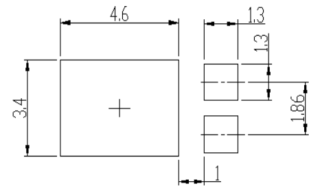
Soldering footprint
